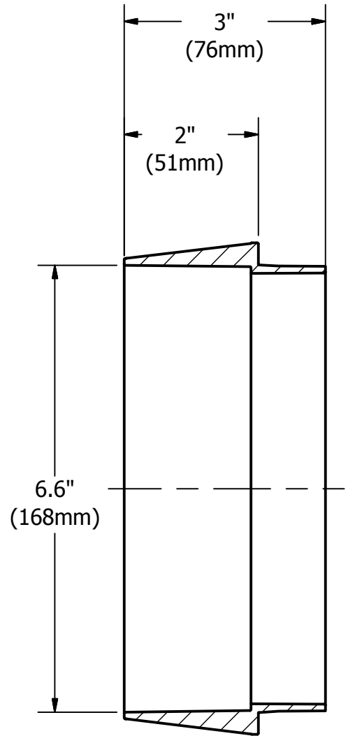
SECTION B-B
